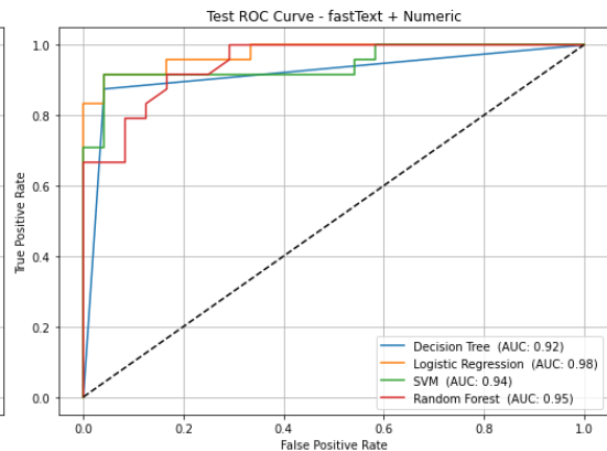
ROC Curves for All Models (Test Set)
