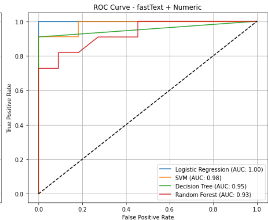
ROC Curves for All Models (Test Set)
